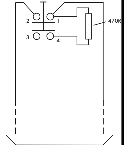
CONNECTIONS FOR UNMONITORED INPUT
