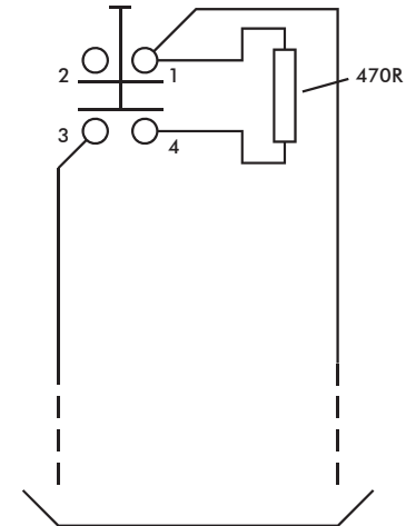
CONNECTIONS FOR MONITORED INPUT
