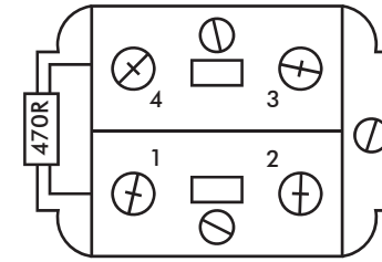
REVERSE VIEW OF CONTACT BLOCK ASSEMBLY
