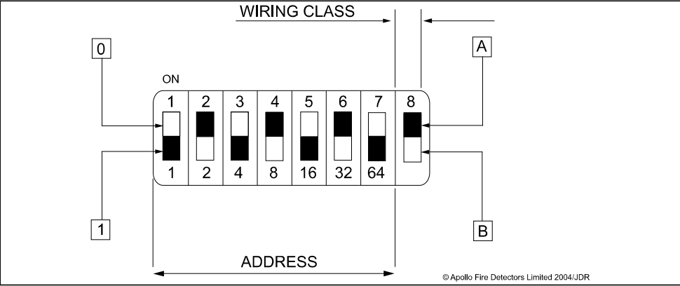
Fig. 2 DIL Switch, S1 When selecting Class A or B wiring using the DIL switch (Fig. 2), please ensure that the module is not powered. If the module is powered, a trouble condition will be reported at the fire alarm control panel. To remove the trouble condition the module must be powered up again in the correct wiring class setting.
