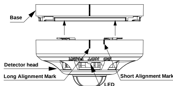
Fig. 3: Fitting the detector to the base
