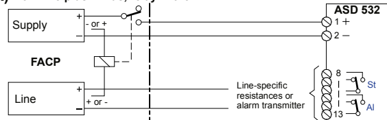
A) from line plus/minus, relay in the ASD
