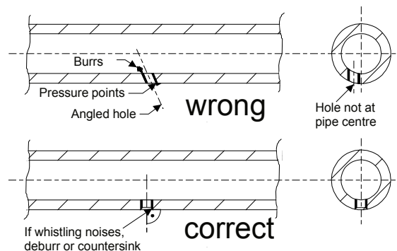
Fig. 12 Creating the sampling holes
