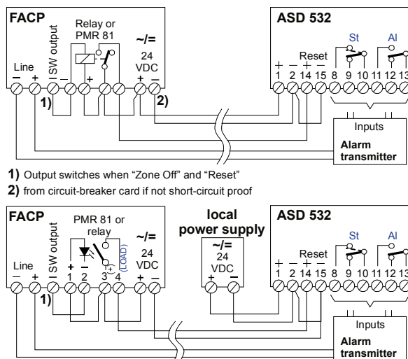
Fig. 24 Connection on selective identification or addressable loop
