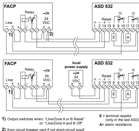
Fig. 23 Connection to zone detection
