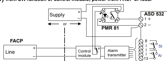
Fig. 21 Control via supply with relay
