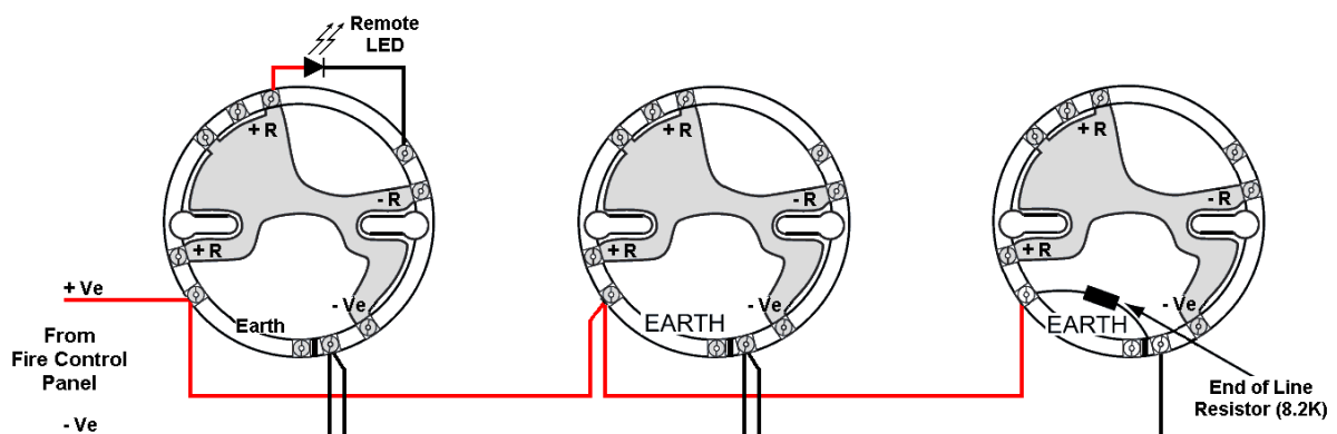
Figure 6 - Wiring diagram for Sav-Wire Base
