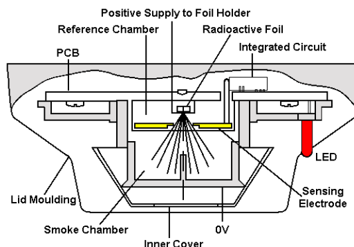
Figure 1 - Side View, Series 65 Ionisation Smoke Detector
